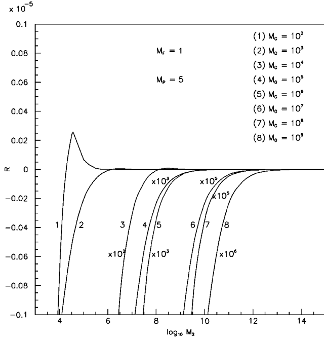
FIG. 2. The ratio R \equiv m_\nu / m_N [Eq. (23)] as a function of M_2 (in units of M_F , and hence the notation M_F=1 ), for M_P=5 and for various values of M_G . For visibility purpose, a few curves have been inflated by factors \times 10^{2,3,5,6} .
