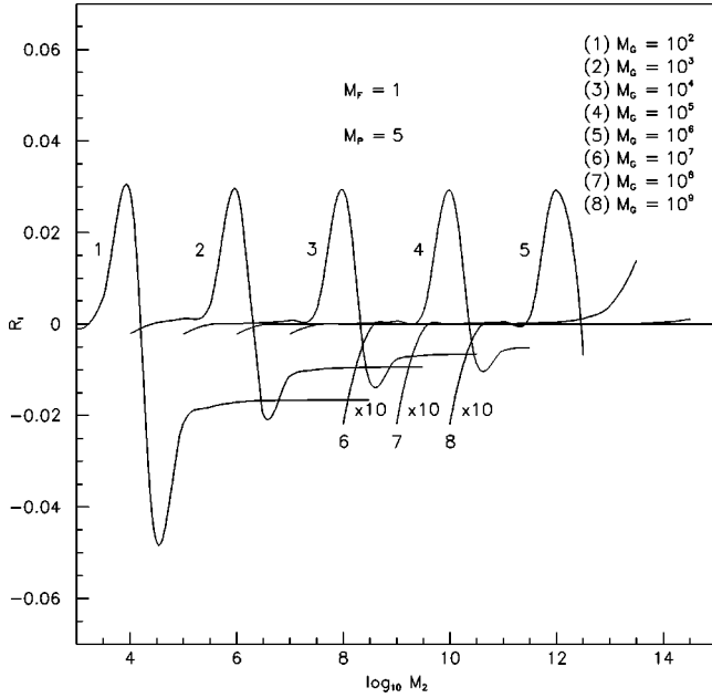
FIG. 7. The ratio R_l \equiv \Delta I(G, P, x_l) / \Delta I(G, P) for b = 0.000095 .
