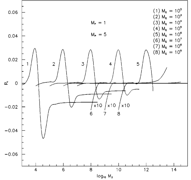
FIG. 6. The ratio R_I \equiv \Delta I(G, P, x_i) / \Delta I(G, P) for b = 0.035 .
